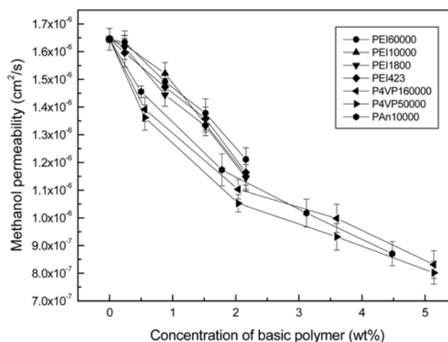
Fig. 7. Methanol permeability according to concentration of base polymer.
